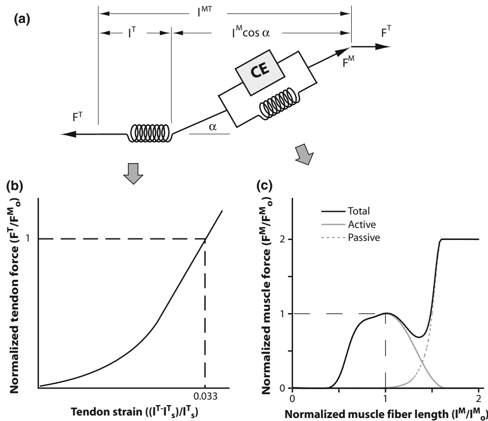
FIGURE 3. Hill-type model of muscle used to estimate tendon and muscle force. (a) The muscle–tendon length ( l^{MT} ) derived from the muscle–tendon geometry was used to compute muscle fiber length ( l^M ), tendon length ( l^T ), pennation angle ( \alpha ), muscle force ( F^M ), and tendon force ( F^T ). (b) Tendon was represented as a non-linear elastic element. We assumed that the strain in tendon ( (l^T - l_s^T)/l_s^T ) was 0.033 when muscle generated maximum isometric force ( F_o^M ). Muscle was represented as a passive elastic element in parallel with an active contractile element (CE). Normalized active and passive force length curves were scaled by maximum isometric force ( F_o^M ) and optimal fiber length ( l_o^M ) derived from experimental measurements for each muscle.
