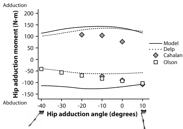
FIGURE 9. Maximum isometric hip adductor moments over a range of hip adduction angles. Adduction moments and angles are positive; abduction moments and angles are negative. The moments estimated with the model were compared to a previous model described by Delp et al. 13 and experimental data reported by Cahalan et al. 8 and Olson et al. 33
