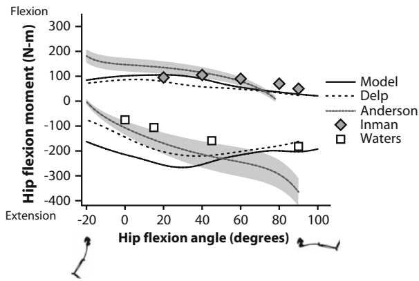
FIGURE 8. Maximum isometric hip flexion moments over a range of hip flexion angles. Flexion moments and angles are positive; extension moments and angles are negative. The moments estimated with the model were compared to a previous model described by Delp et al. 13 and experimental data reported by Anderson et al. , 1 Inman et al. , 23 and Waters et al. 45 The gray region indicates one standard deviation of the data reported by Anderson et al. 1
