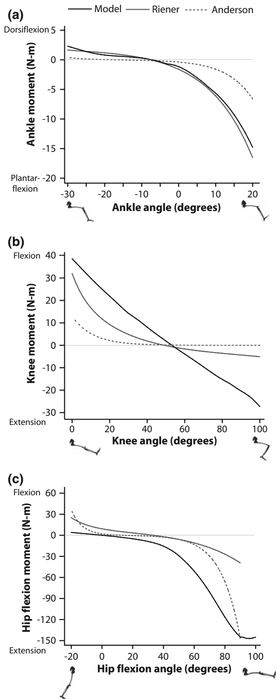
FIGURE 5. Passive joint moments calculated by the model and measured experimentally. Passive joint moment was summed from all muscles crossing each joint and compared to experimental results reported by Riener et al. 37 and Anderson et al. 1 There are no experimental results for passive adduction/abduction moments. The joints of the model were positioned to match those used by Anderson et al. The ankle moment (a) was calculated when knee and hip flexion angles were 80° and 50°. The knee moment (b) was calculated when the hip flexion and ankle angles were 70° and 0°. The hip flexion moment (c) was calculated when the knee angle was 10°.
