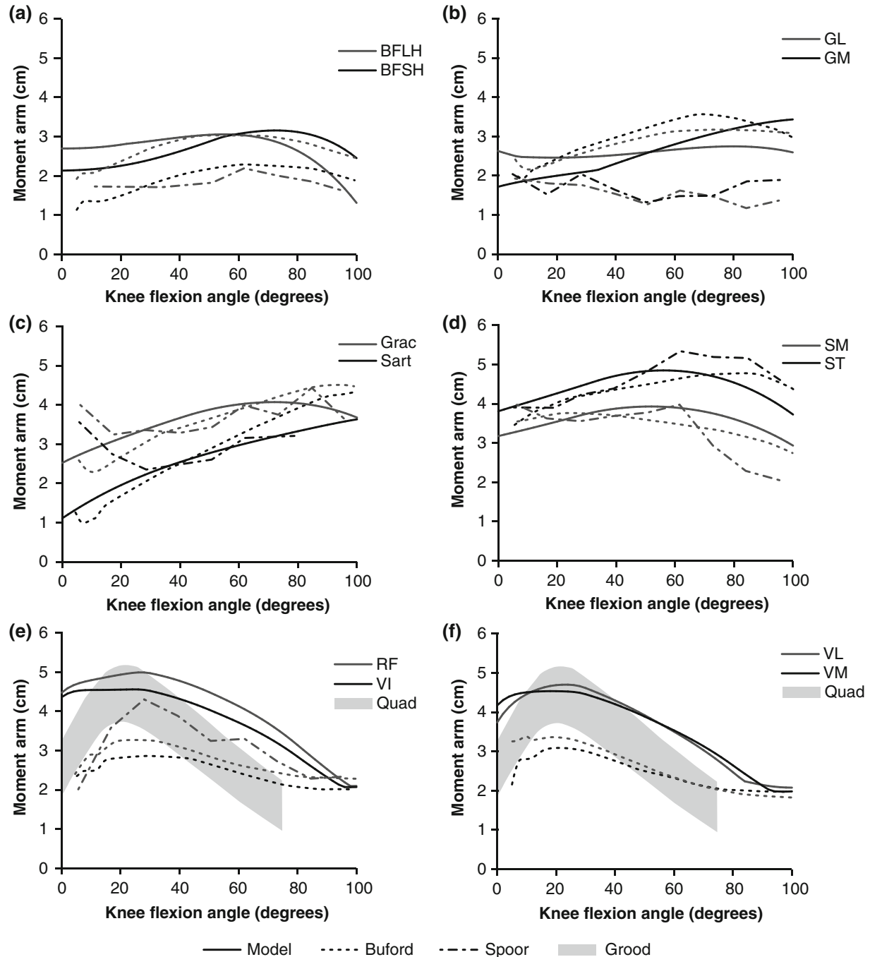
FIGURE 4. Moment arms of muscles crossing the knee in the model (solid), Buford et al. 7 (dashed), Spoor and van Leeuwen 40 (dot-dashed), and Grood et al. 18 (shaded area). Muscle moment arms are shown for (a) biceps femoris long head (BFLH) and biceps femoris short head (BFSH), (b) gastrocnemius lateralis (GL) and gastrocnemius medialis (GM), (c) gracilis (Grac) and sartorius (Sart), (d) semimembranosus (SM) and semitendinosus (ST), (e) rectus femoris (RF), vastus intermedialis (VI), and grouped quadriceps (Quad), and (f) vastus lateralis (VL), vastus medialis (VM), and grouped quadriceps (Quad).
